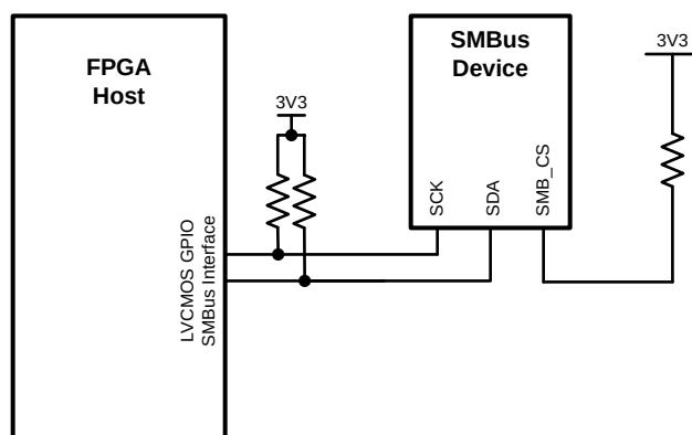
Figure 10. SMBus Configuration 1
