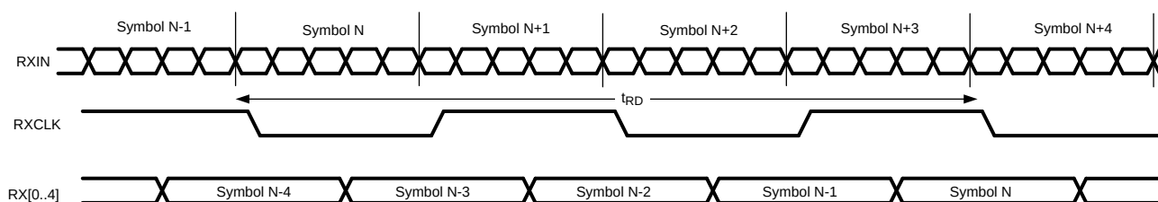
Figure 7. Deserializer Propagation Delay
