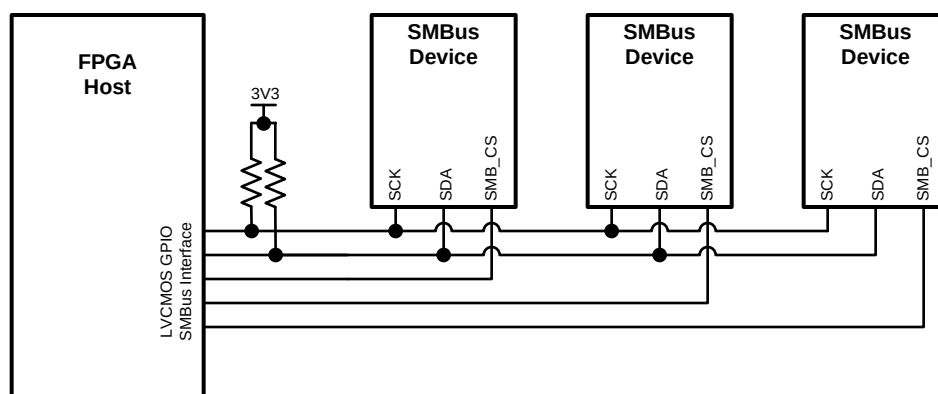
Figure 11. SMBus Configuration 2
