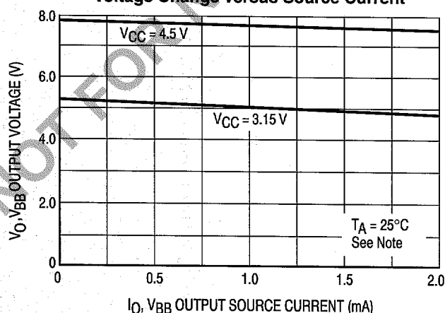
Figure 4. V_BB Output Voltage Change versus Source Current
