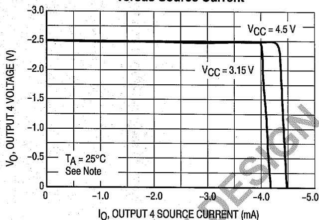
Figure 2. Output 4 Voltage versus Source Current
