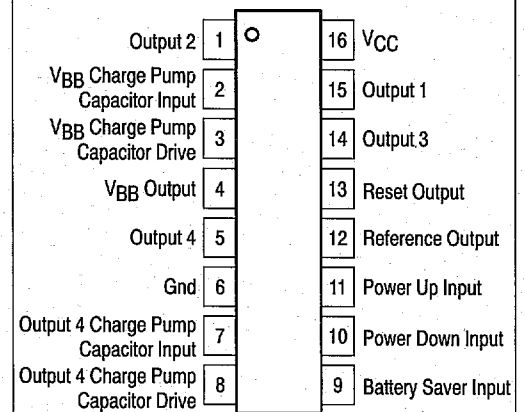
PIN CONNECTIONS
