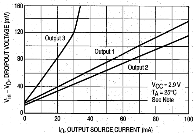
Figure 1. Dropout Voltage versus Source Current
