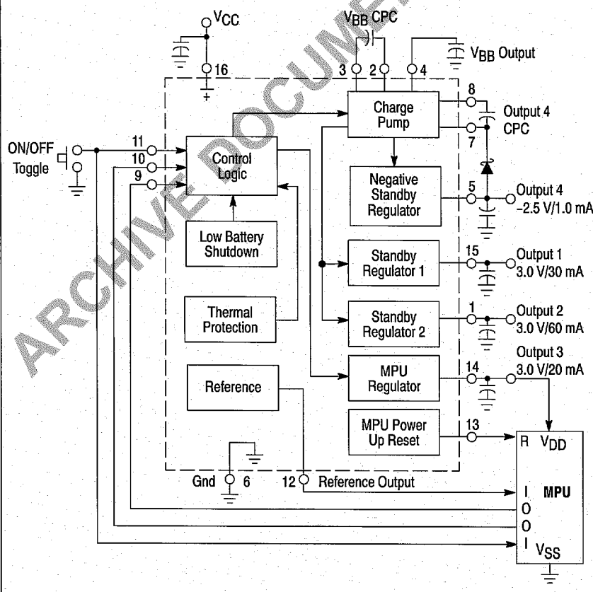
Simplified Block Diagram
