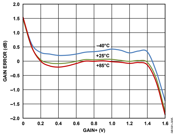
Figure 5. Gain Error vs. GAIN+ at Three Temperatures
