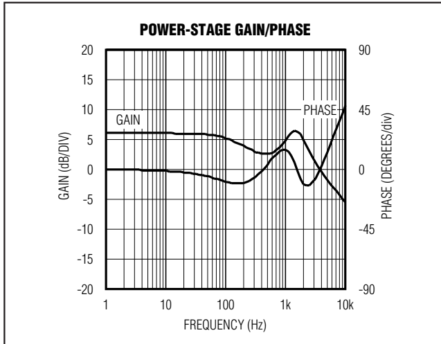
Figure 16. Idealized (with Ideal Power Stage and Optocoupler) Frequency Response ( G_P(s) ) from Noninverting Input of the Error Amplifier to the Output of the Power Supply for the Typical Application Circuit of Figure 18
