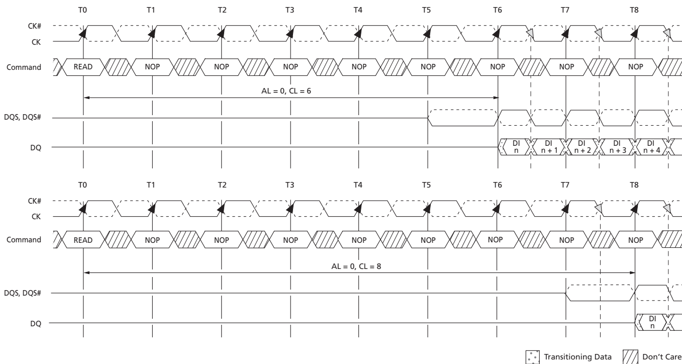
Figure 53: READ Latency
