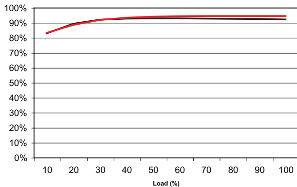
Figure 8 - AHM180PS24
