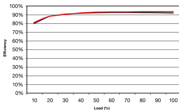
Figure 7 - AHM85PS12
