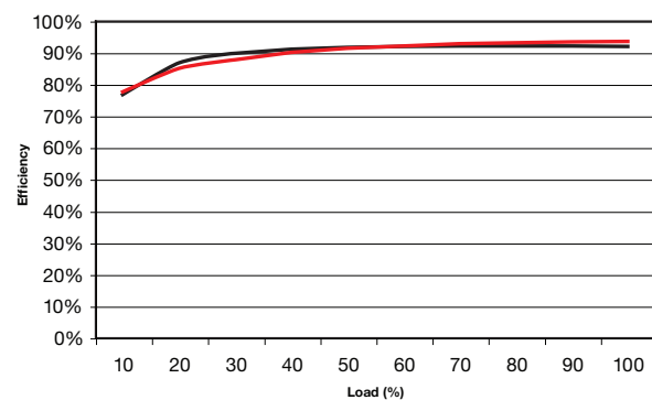
Figure 8 - AHM85PS24
