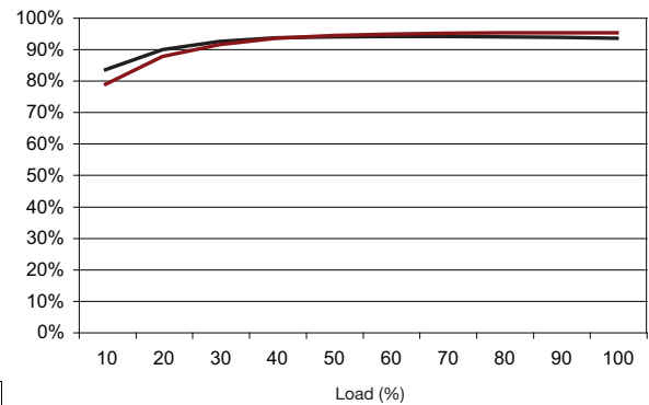
Figure 10 - AHM250PS48
