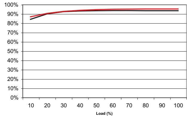
Figure 9 - AHM180PS48
