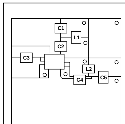
Figure 23. Eight-Pin SOIC Layout, Component Placement Diagram (1x Scale)
