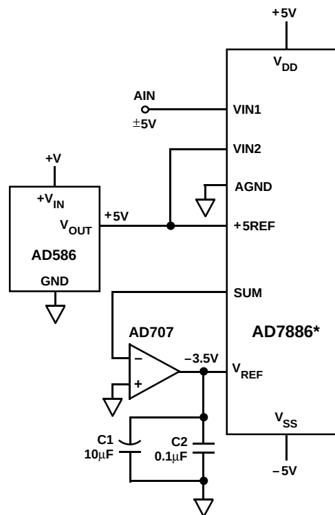
Figure 7. Bipolar Operation
