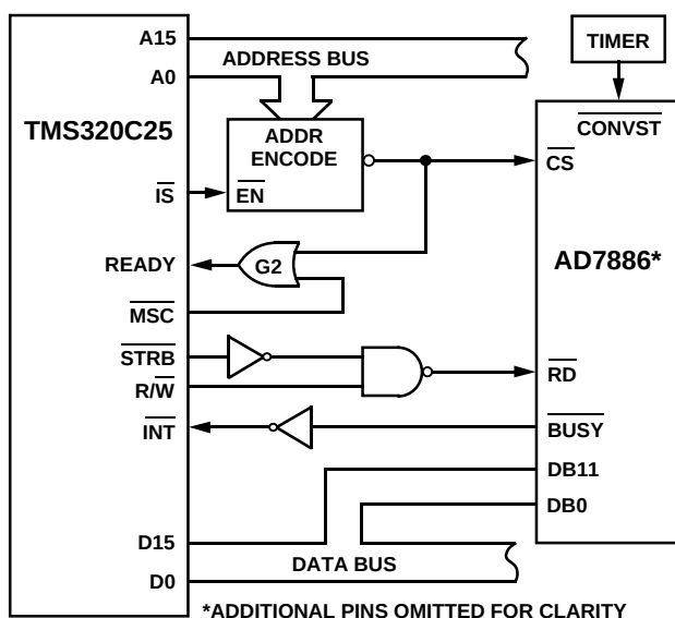
Figure 18. AD7886-TMS320C25 Interface
