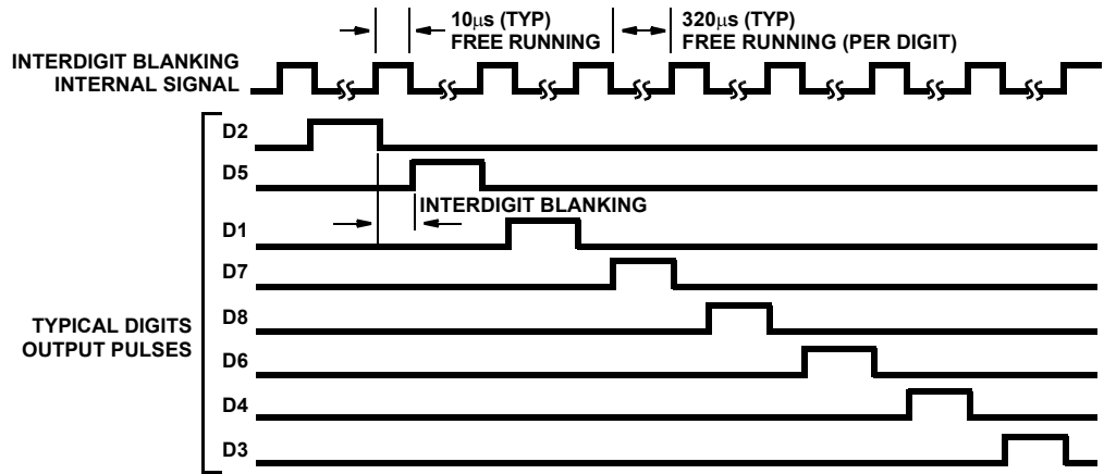
FIGURE 4. DISPLAY DIGITS MULTIPLEX (COMMON ANODE DISPLAY)
