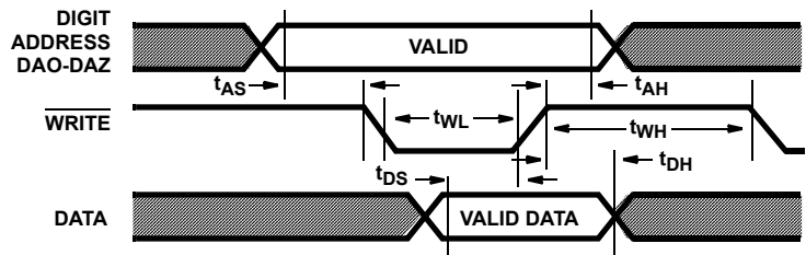
FIGURE 3. ICM7228C WRITE CYCLE
