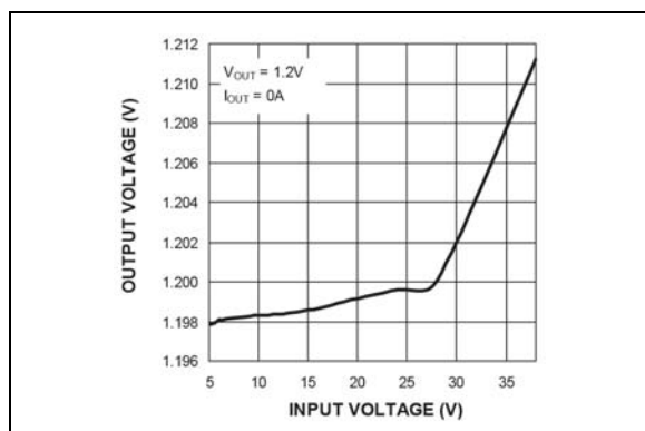
FIGURE 2-7: Output Voltage vs. Input Voltage (MIC2101).
