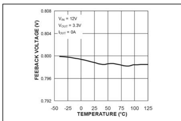
FIGURE 2-9: Feedback Voltage vs. Temperature (MIC2101).
