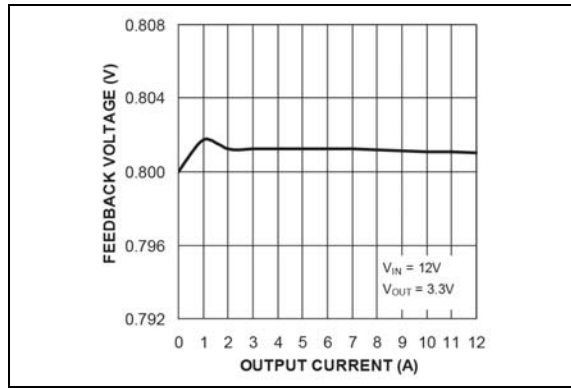
FIGURE 2-12: Feedback Voltage vs. Output Current (MIC2101).
