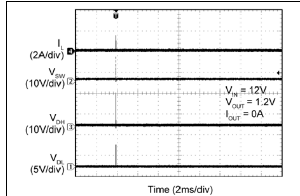
FIGURE 2-88: MIC2101 Switching Waveforms ( I_{OUT} = 0A ).
