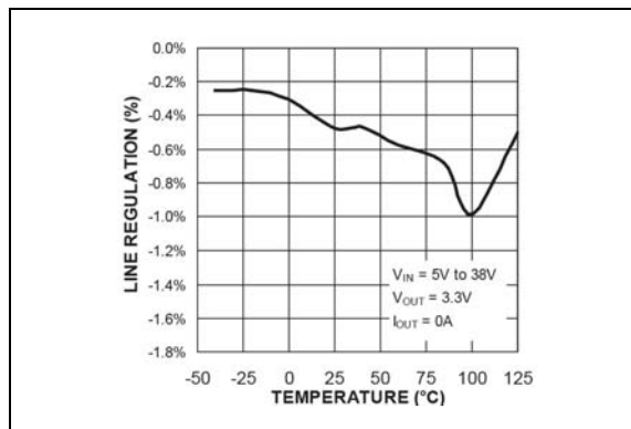
FIGURE 2-11: Line Regulation vs. Temperature (MIC2101).
