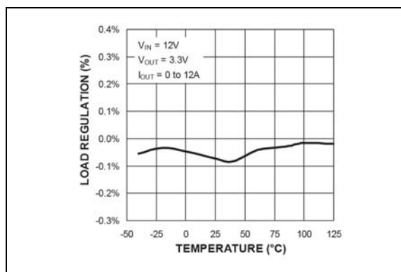
FIGURE 2-10: Load Regulation vs. Temperature (MIC2101).
