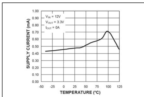
FIGURE 2-8: VIN Operating Supply Current vs. Temperature (MIC2101).
