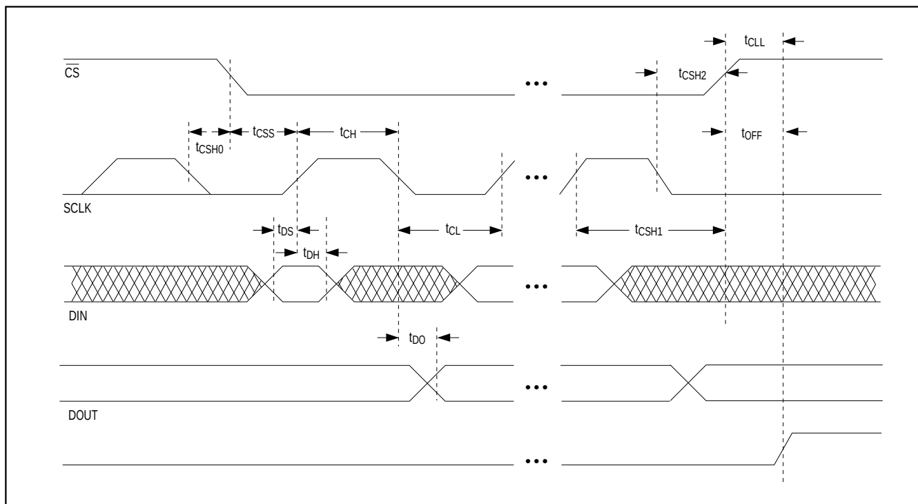
Figure 1. Timing Diagram
