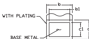
LEAD TIP DETAIL
