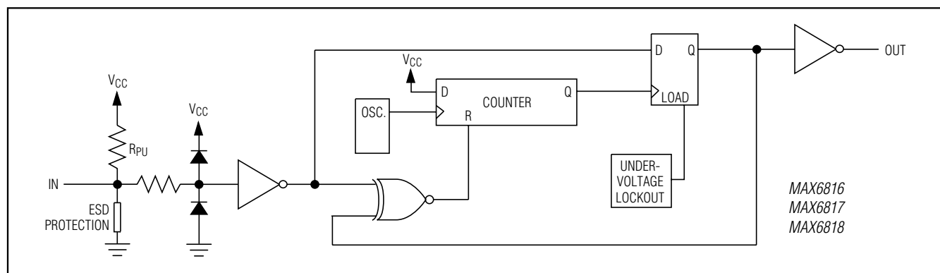
Figure 1. Block Diagram
