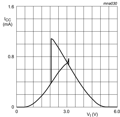
Fig. 11. Typical 74HC1G14-Q100 transfer characteristics; V_{CC} = 6.0\text{ V}
