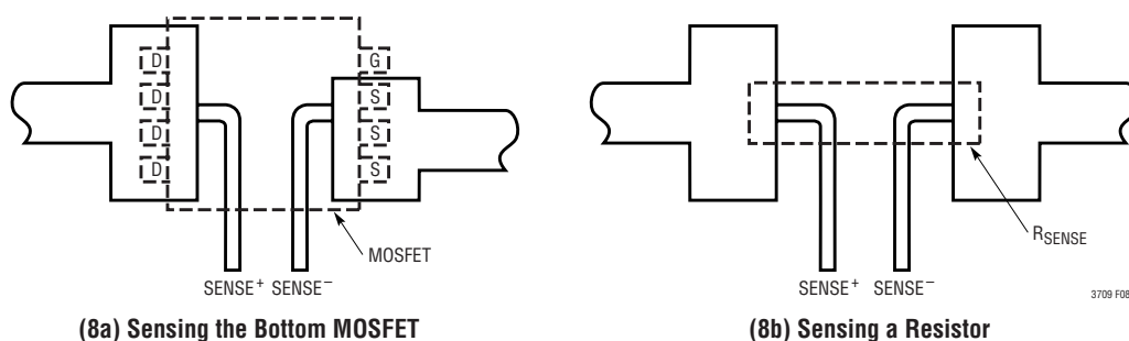
Figure 8. Kelvin Sensing
