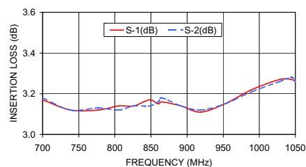
ZN2PD-920W INSERTION LOSS
