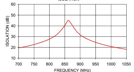
ZN2PD-920W ISOLATION
