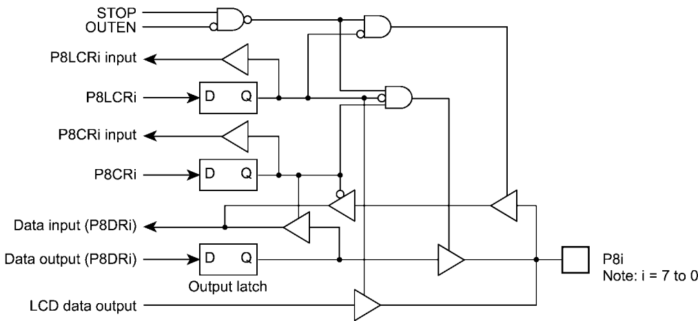
Figure 5-8 Port P8
