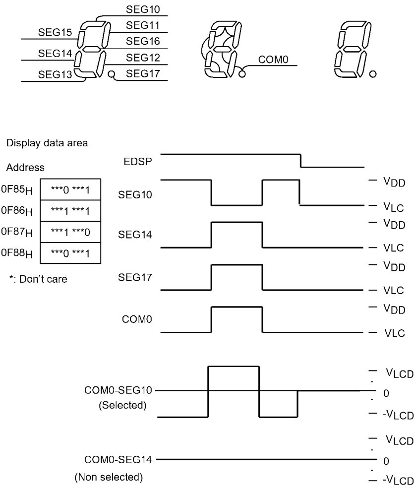
Figure 15-11 Static Drive
