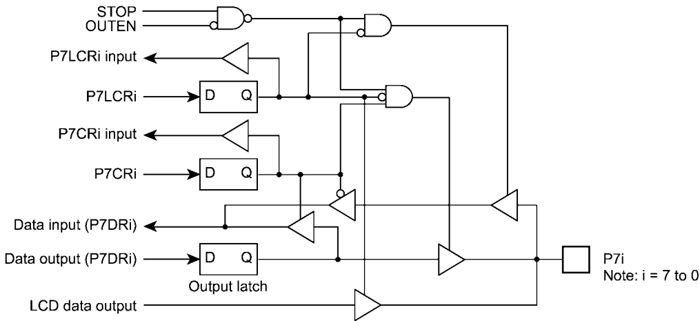
Figure 5-7 Port P7
