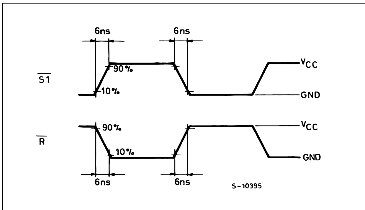
INPUT WAVEFORMS ( f=1\text{MHz} ; 50% duty cycle)
