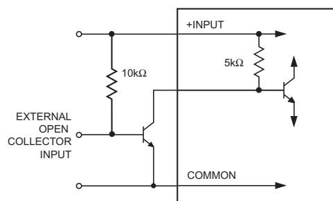
External Input Open: On/Off pin Low = DC/DC converter Off External Input Low: On/Off pin High = DC/DC converter On
