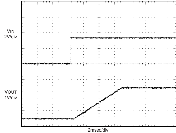
Start-Up from VIN (IOUT = 2V/10A, CIN/COUT = 22μF)
