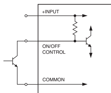
ON/OFF pin open: Logic High = DC/DC converter On ON/OFF pin <0.4V: Logic Low = DC/DC converter Off
