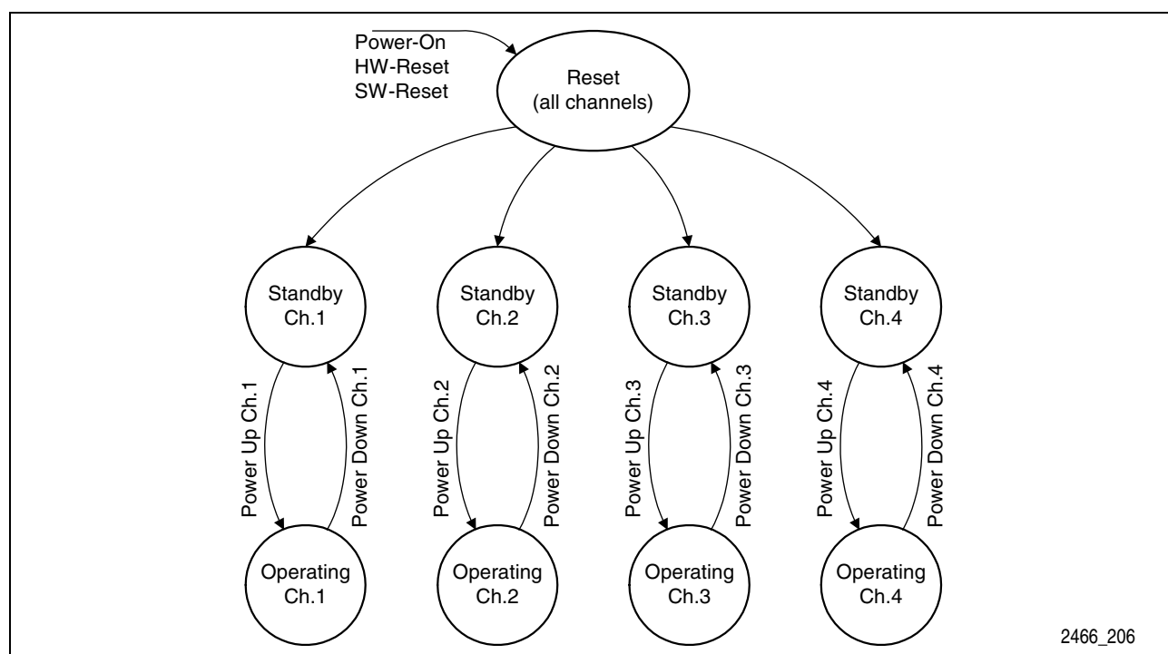
Figure 5 SICOFI®4-μC State Diagram
