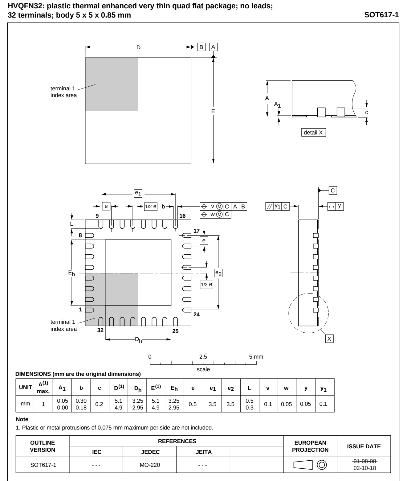
Fig 30. Package outline SOT617-1 (HVQFN32)
