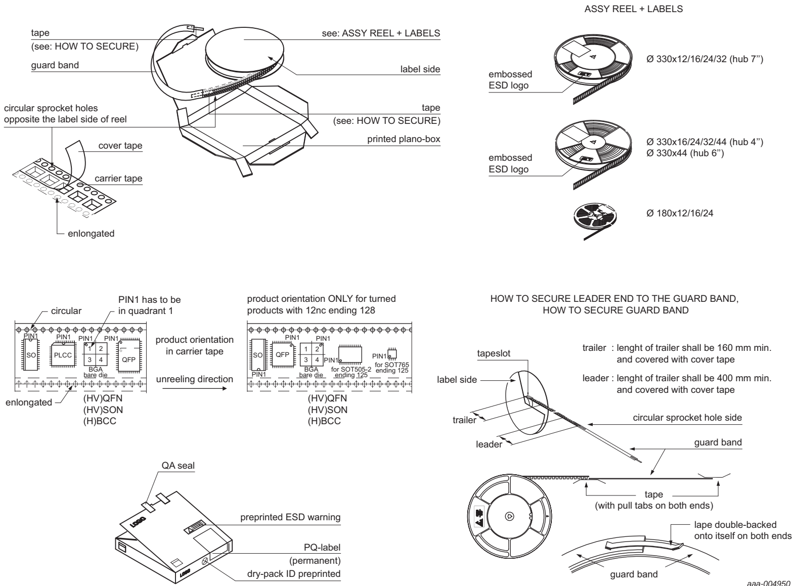
Fig 34. Packing information Reel
