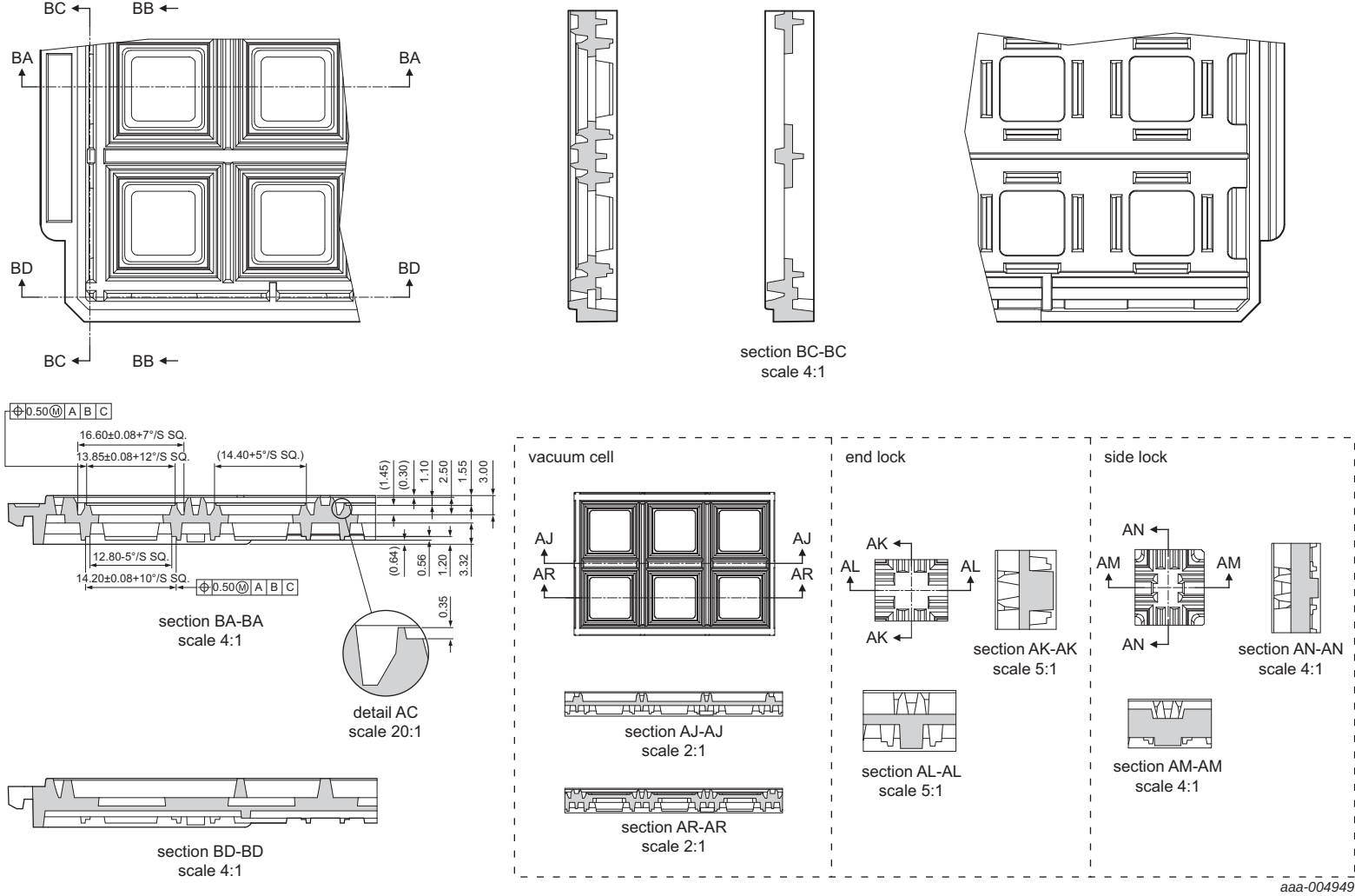
Fig 33. Tray details
