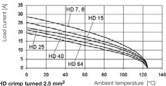
HD crimp turned 2.5 mm 2 Ambient temperature [°C]
