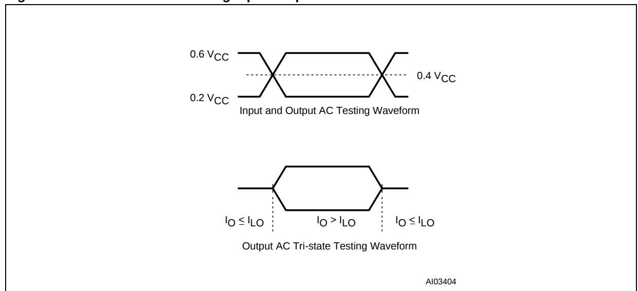
Figure 7. LPC Interface AC Testing Input Output Waveforms
