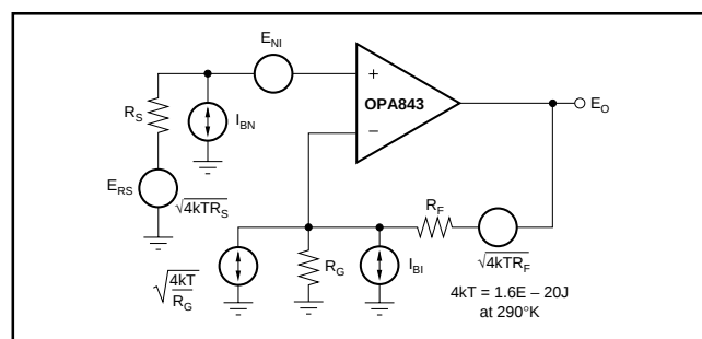
Dividing this expression by the noise gain ( NG = 1 + R_F/R_G ) will give the equivalent input referred spot noise voltage at the noninverting input, as shown in Equation 16.
