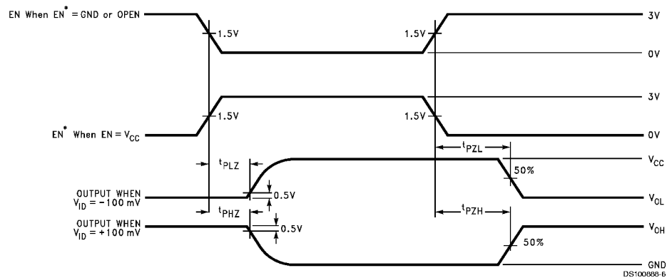
FIGURE 4. Receiver TRI-STATE Delay Waveforms
