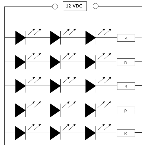
Normal Bright Maximum Length is 12 meters, 360 LEDs
