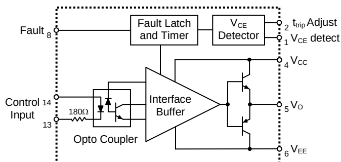
Figure 1: VLA503-01/VLA504-01/M57159L-01 Block Diagram
