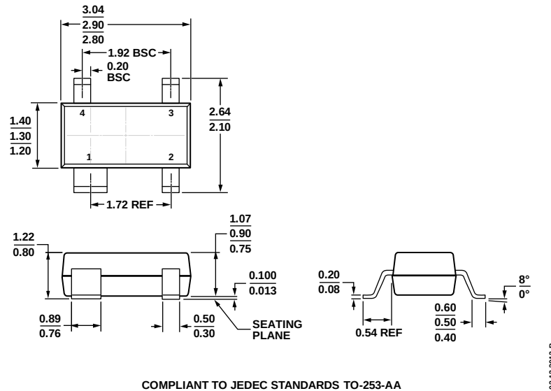
COMPLIANT TO JEDEC STANDARDS TO-253-AA Figure 12. 4-Lead Small Outline Transistor Package [SOT-143] (RA-4) Dimensions shown in millimeters
