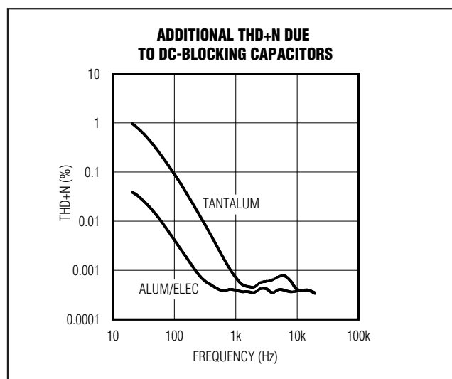
Figure 3. Distortion Contributed by DC-Blocking Capacitors
