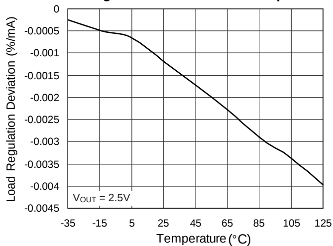
Load Regulation Deviation vs. Temperature
