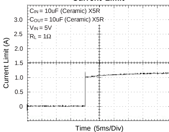
Current Limit
