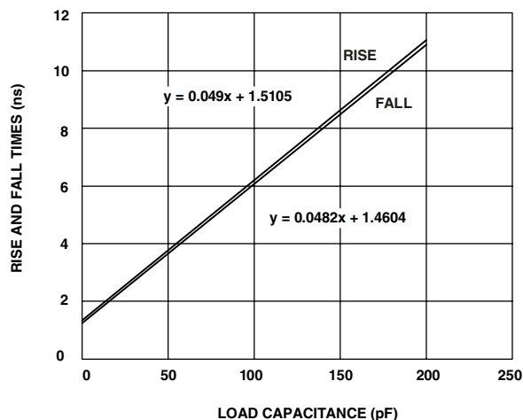
Figure 40. Typical Output Rise/Fall Time (20%-80%, V_{DDEXT} = \text{Min} )
