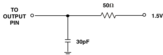
Figure 37. Equivalent Device Loading for AC Measurements (Includes All Fixtures)
