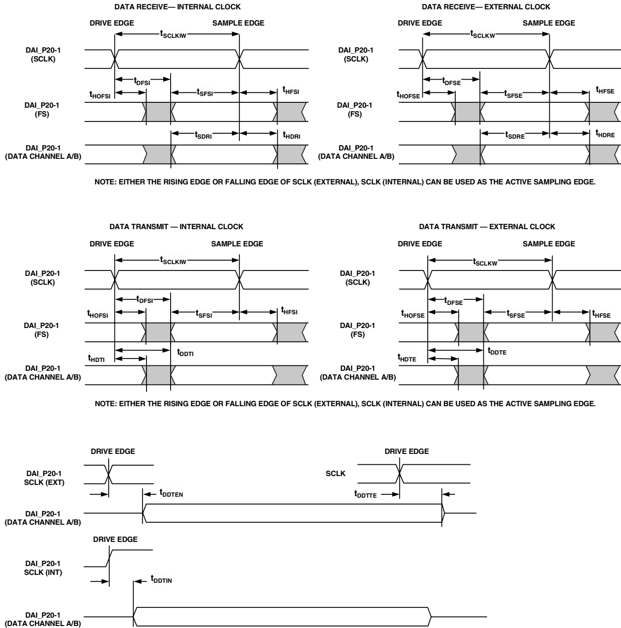
Figure 22. Serial Ports
