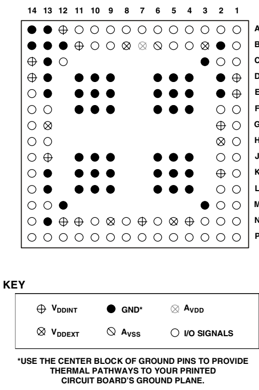
Figure 42. 136-Ball Mini-BGA Pin Assignments (Bottom View, Summary)
