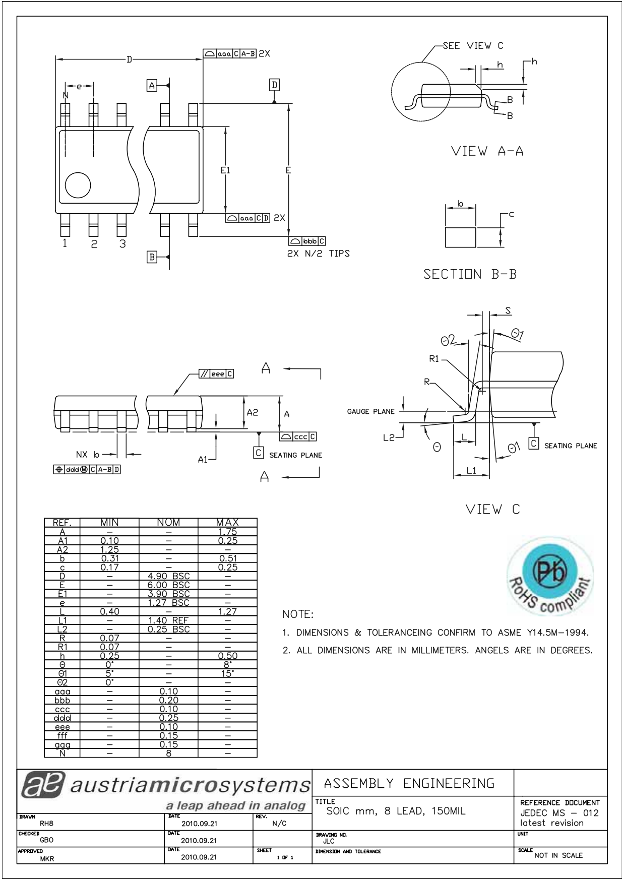
Figure 23. 8-pin SOIC Package Diagram
