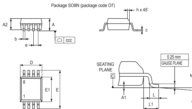
Figure 19. SO8N – Outline
