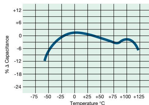
Temperature Coefficient
