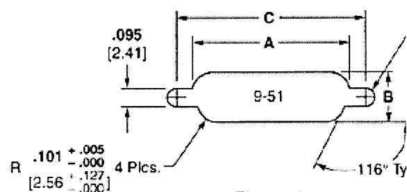
Figure 2 Rear Mounting
