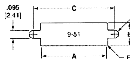
Figure 1 Front Mounting
