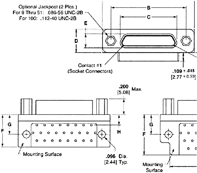
9, 15, 21 & 25 Contacts
