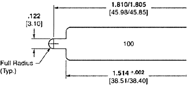
Rear Mounting
