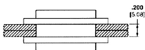
Plug and Receptacle Rear Mounted
