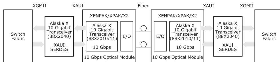
Fig 2. Alaska X 10 Gigabit Transceiver (88X2010/88X2011) Applications Diagram
