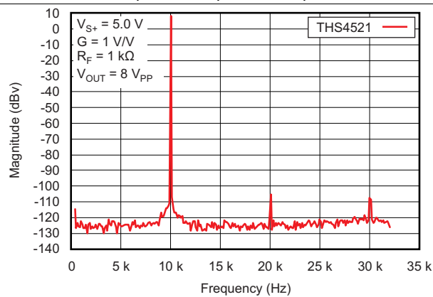
Figure 33. 10-kHz Output Spectrum On AP Analyzer at V_{OUT} = 8\text{ V}_{PP}
