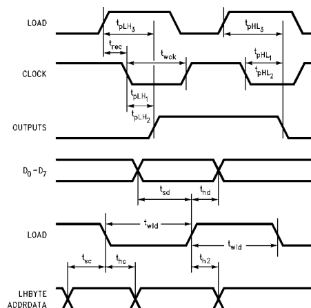
FIGURE 5. AC Specifications
