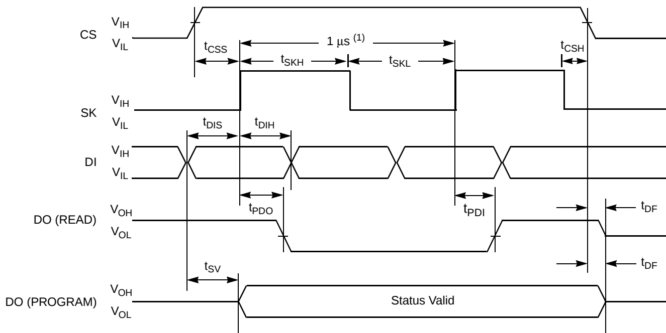
Typical XXC56 Series Serial EEPROM Control Timing
