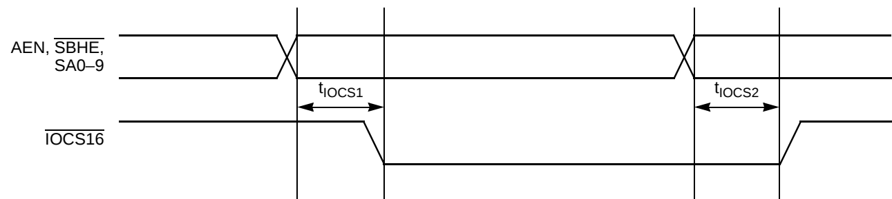
\overline{I/OCS16} Timings
