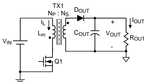
Figure 1. Typical Flyback Converter
