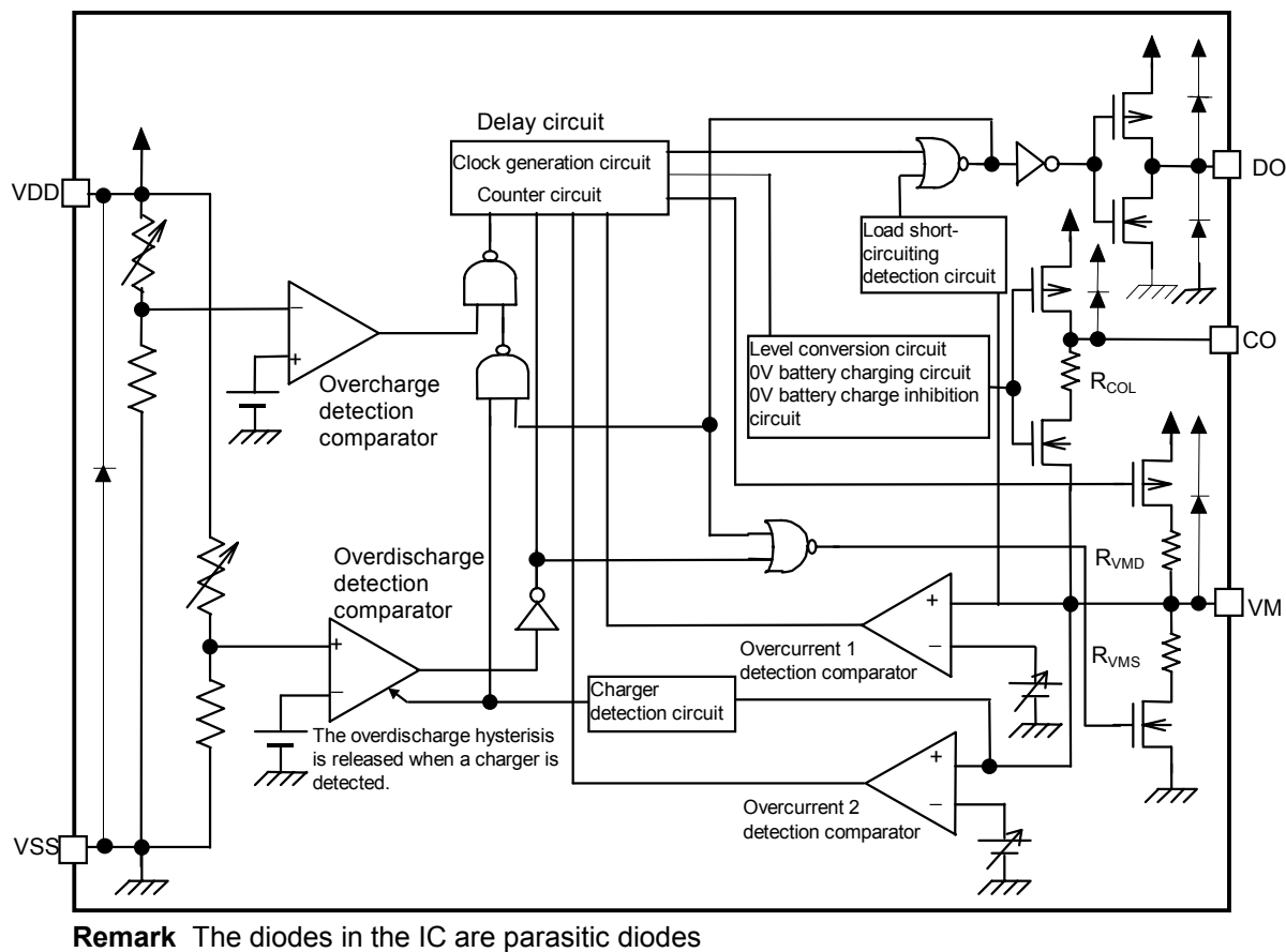
Figure 1 Block Diagram
