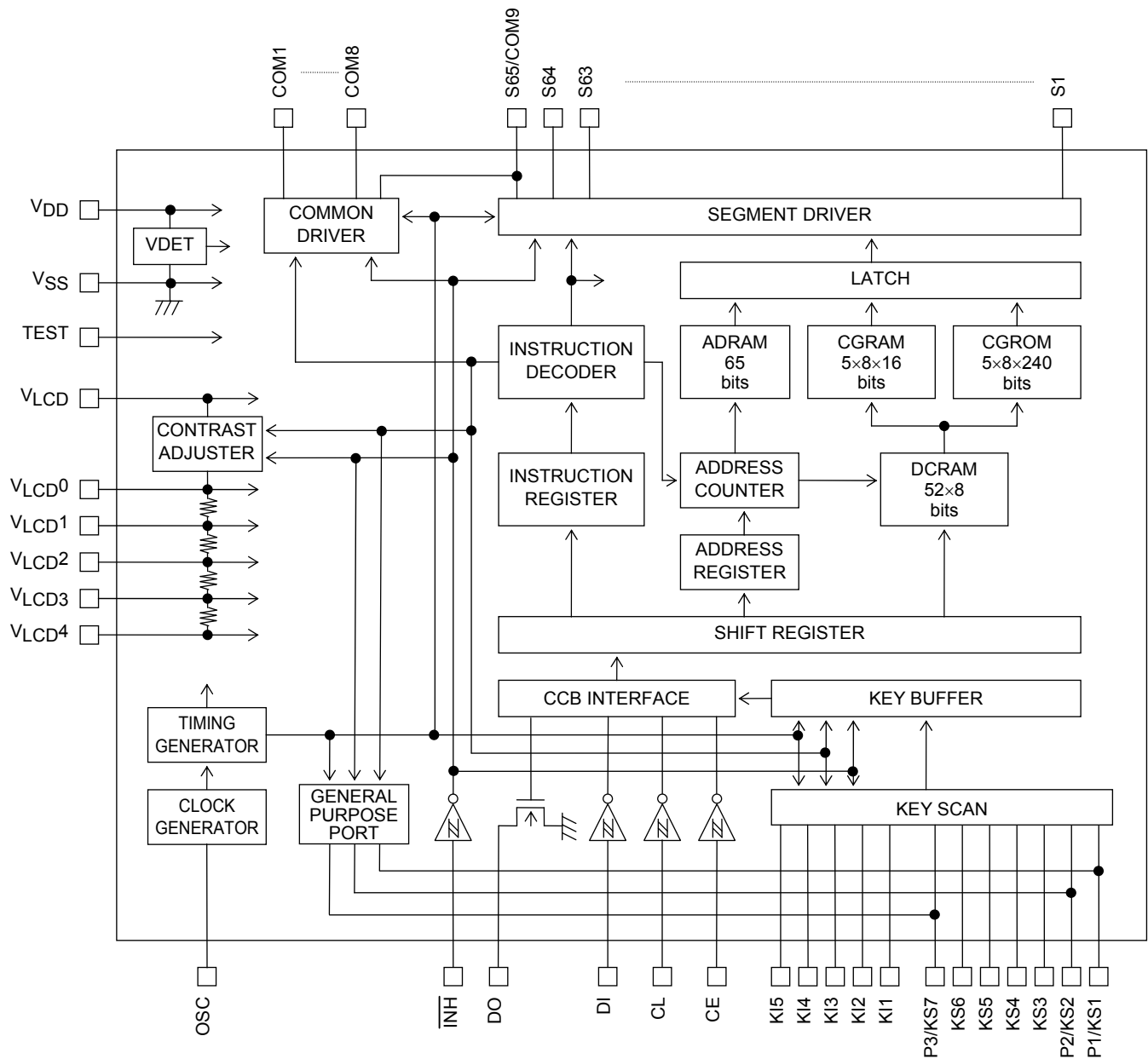
Block Diagram
