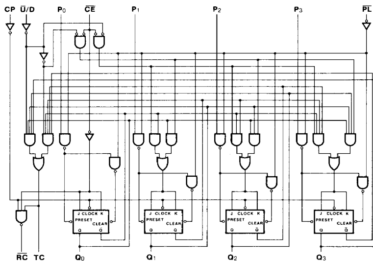
LOGIC DIAGRAM
