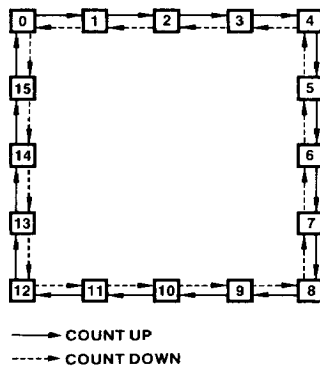
STATE DIAGRAM
