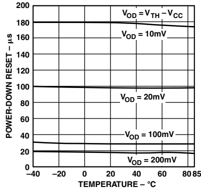
TPC 2. Power-Down RESET Delay vs. Temperature ADM8_L/M/J
