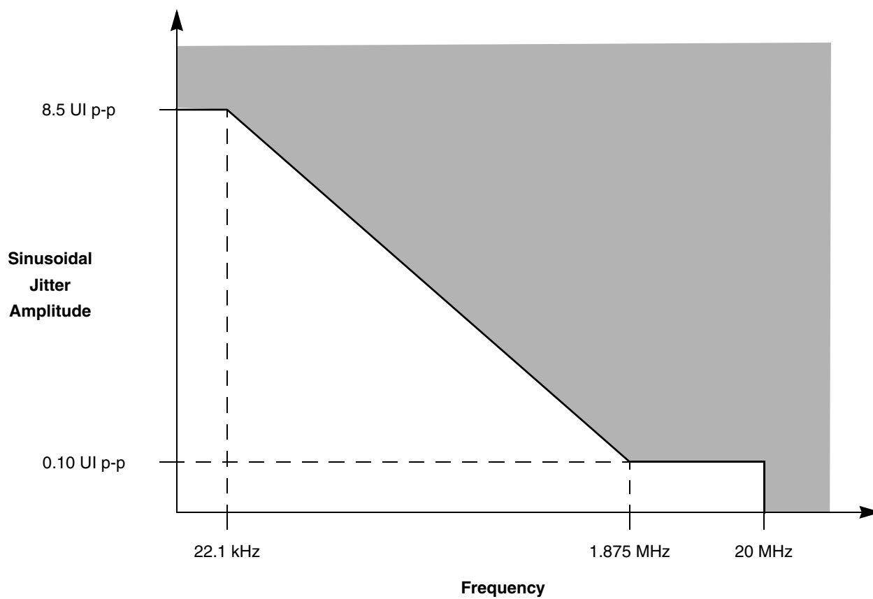
Figure 55. Single Frequency Sinusoidal Jitter Limits
