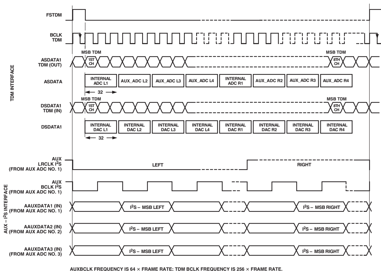
Figure 11. Auxiliary Mode Timing
