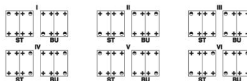
Coding for housings with two contact inserts
