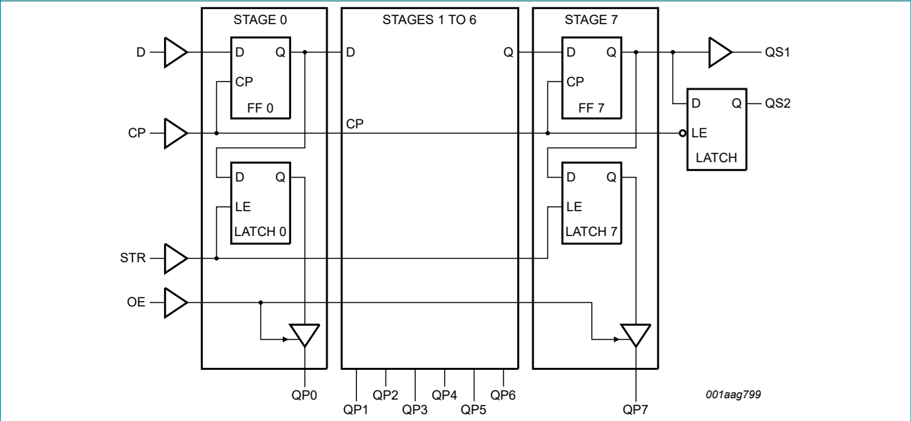
Fig. 4. Logic diagram
