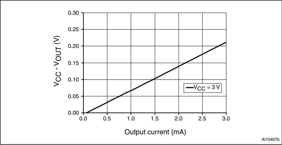
Figure 17. Voltage output high vs. I_{SOURCE}
