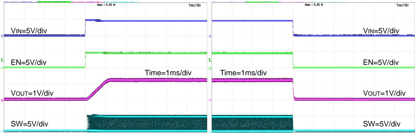
Figure 31. Power Down Waveform with VIN (FREQ=H, RLOAD=0.5Ω)
