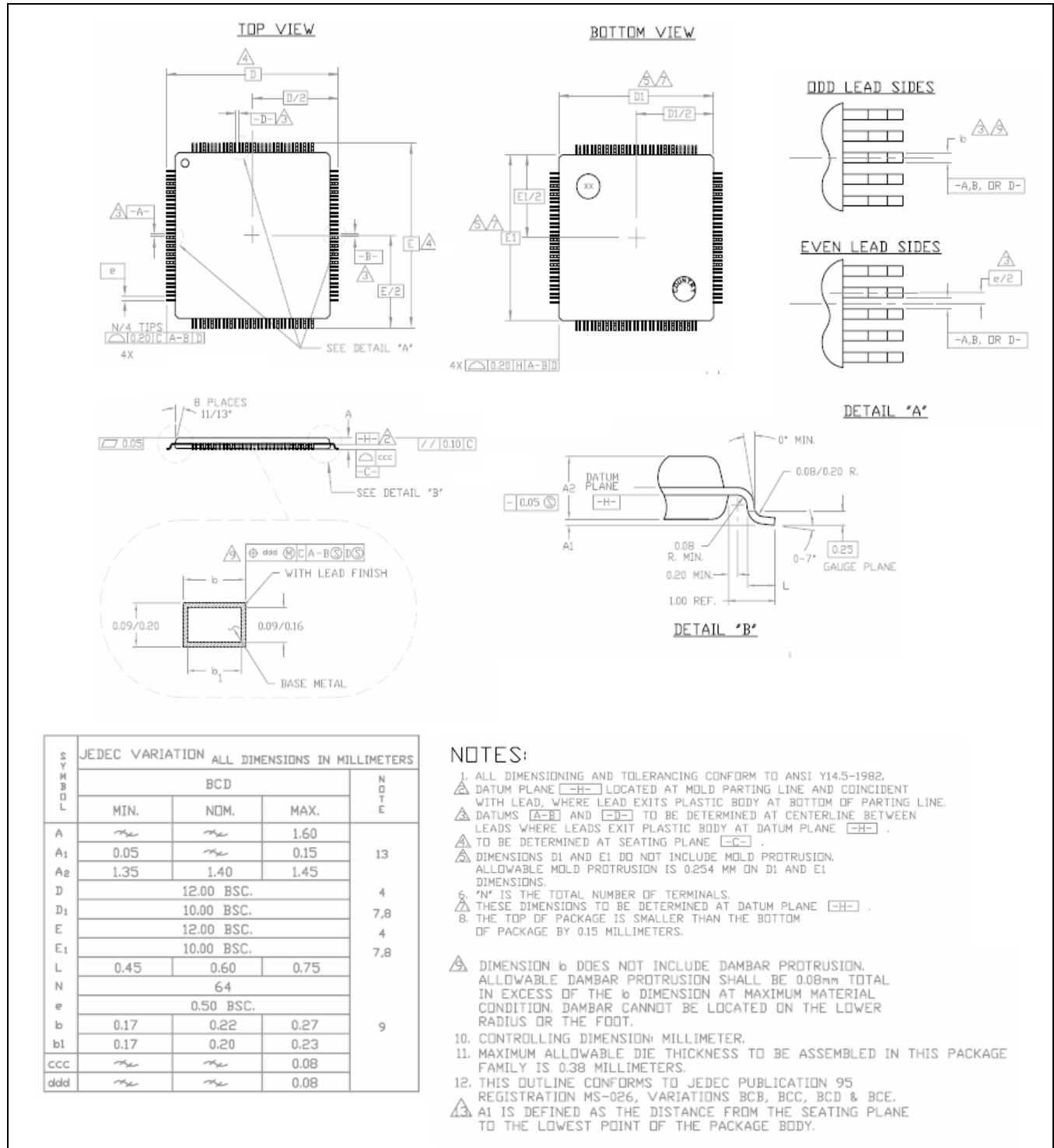
Figure 2-2. Package Drawing
